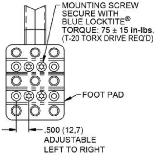
FOOT PAD DETAIL
